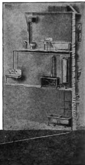
FIG. 216.—Gravity system with ram. Tank located in the attic.
