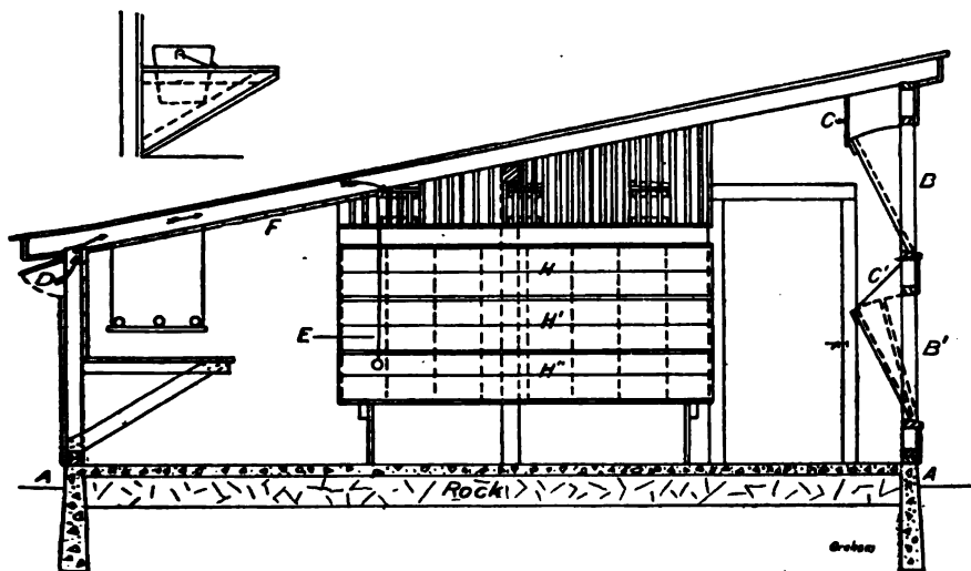
FIG. 134.—Laying house.
