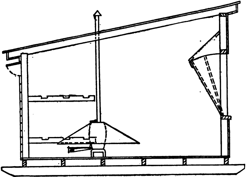
FIG. 135.—Colony house.
