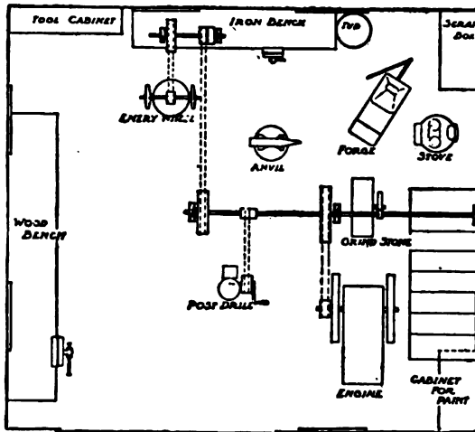
FIG. 225.—Floor plan of the repair shop.
