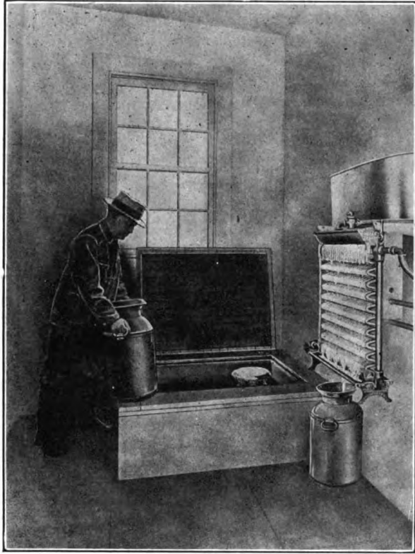
FIG. 169.—Insulated concrete cooling tank partially sunk in the cement floor; also a surface cooler in operation.
