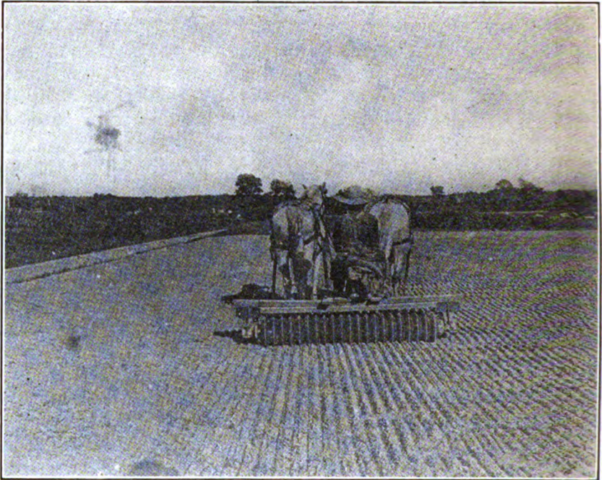
FIG. 24.—Soil in good tilth. The Meeker harrow is a very efficient pulverizing tool. It consists of a series of small disks fitted rigidly to a straight axle. — Indiana Experiment Station, Farmers Bulletin 202.
