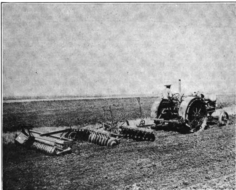
FIG. 4.—Cutting, pulverizing and compacting the seedbed at one operation.— By permission of Dunham Co., Berea, Ohio.
