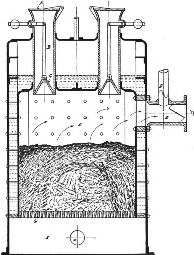
FIG. 16. — BEAUFUME PRODUCER.
