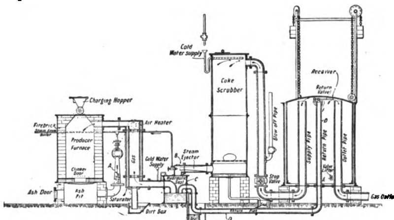
FIG. 48. — SECTION OF WILE AUTOMATIC GAS-PRODUCER.
