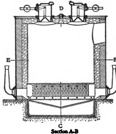
FIG. 31. — DUFF GAS-PRODUCER.
