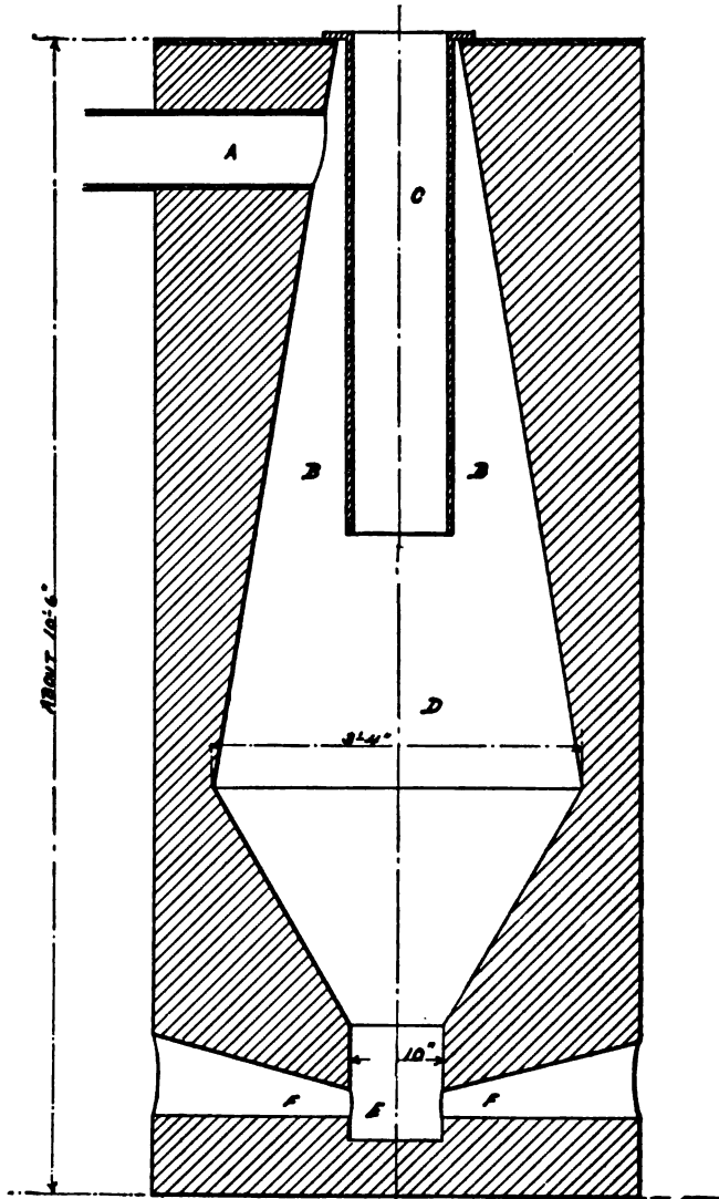
FIG. 13. — EBELSEN PRODUCER.
