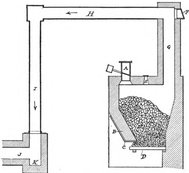
FIG. 18. — SIEMENS GAS-PRODUCER.
