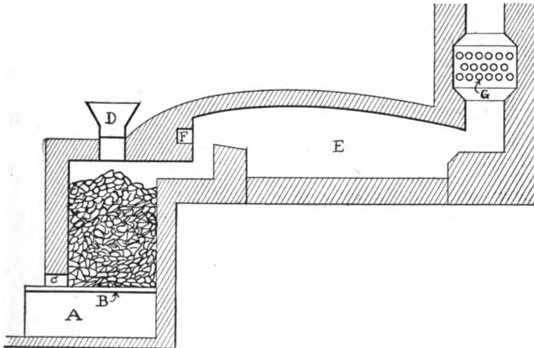
FIG. 12. — EBELMEN GAS-PRODUCER.
