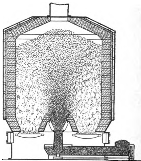
FIG. 106. — SECTION OF CAPITAINE SOFT-COAL PRODUCER. (Courtesy of Engineering Magazine .)
