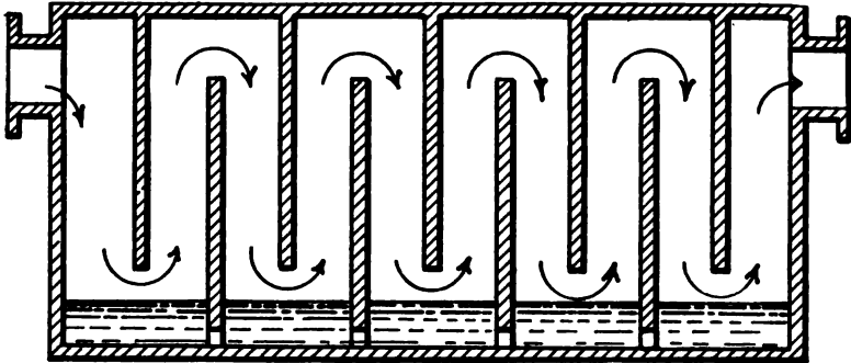
FIG. 72. — MOISTURE COLLECTOR.
