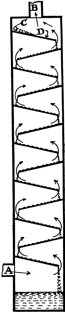
FIG. 77. FILM SCRUBBER.
