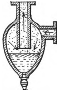
FIG. 74. — MOISTURE COLLECTOR.
