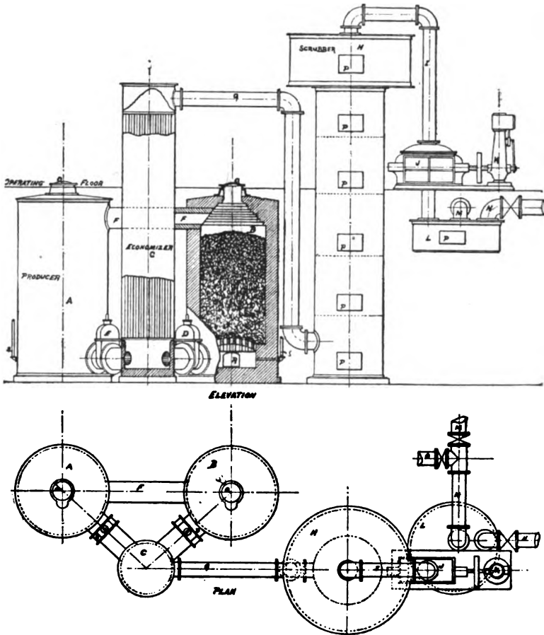
FIG. 47. — LOOMIS GAS-PRODUCER.
