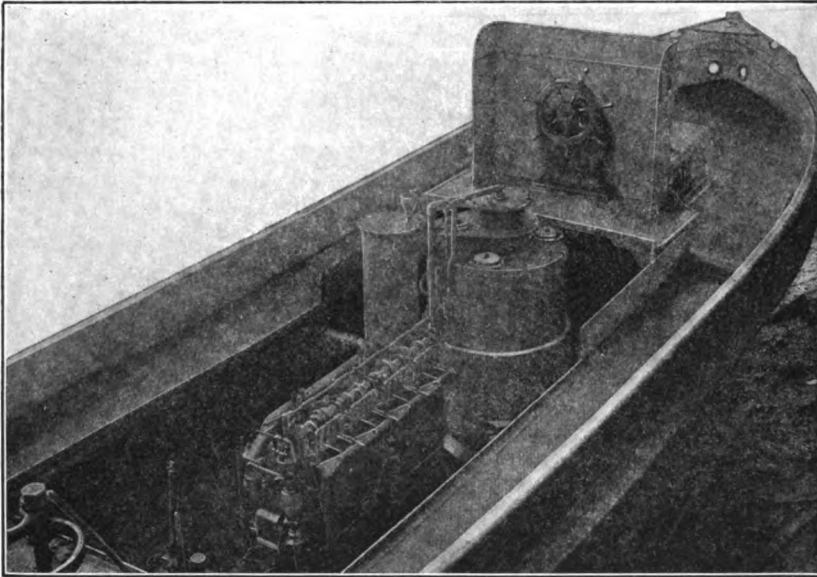
FIG. 111. — PRODUCER-GAS-ENGINE-DRIVEN TUGBOAT.
