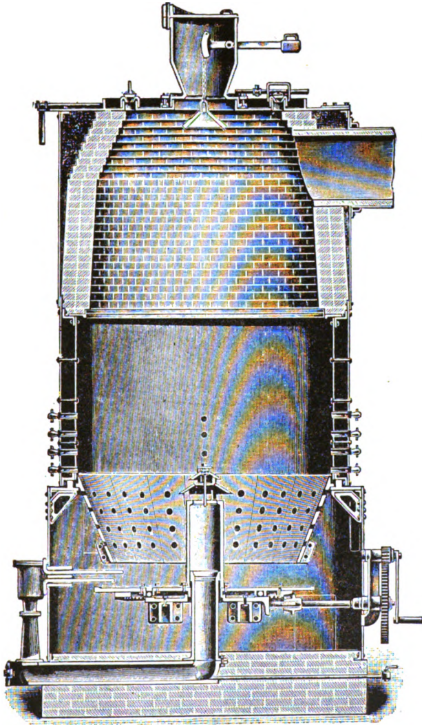
FIG. 34. — SECTION OF TAYLOR GAS-PRODUCER.
