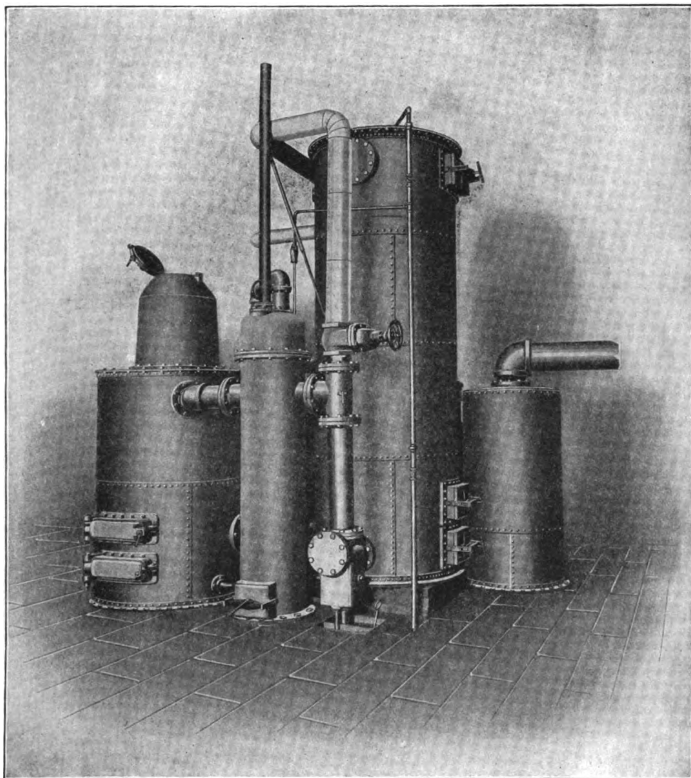
FIG. 52. — OTTO SUCTION GAS-PRODUCER.
