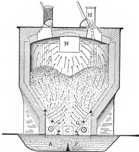
FIG. 26. — SWINDELL GAS-PRODUCER.
