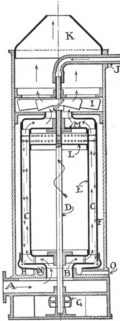
FIG. 79. — SECTION OF WINDHAUSEN GAS-SCRUBBER.
