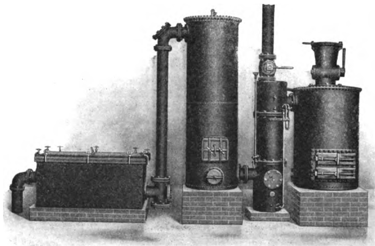
FIG. 55. — WILE SUCTION GAS-PRODUCER.
