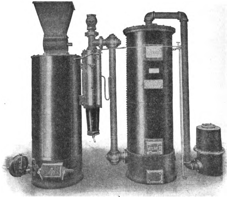
Blower. Producer Vaporizer. Scrubber. Receiver. FIG. 53. — WEBER SUCTION GAS-PRODUCER.
