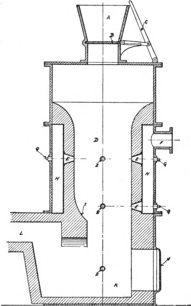
FIG. 15. — EKMAN PRODUCER.
