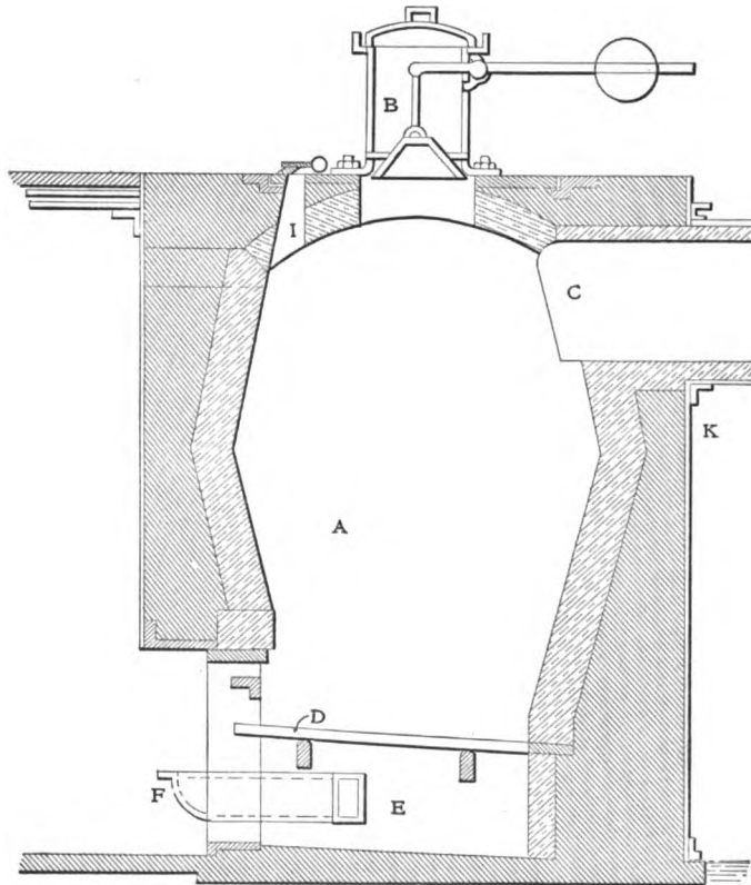
FIG. 41. — WELLMAN GAS-PRODUCER.
