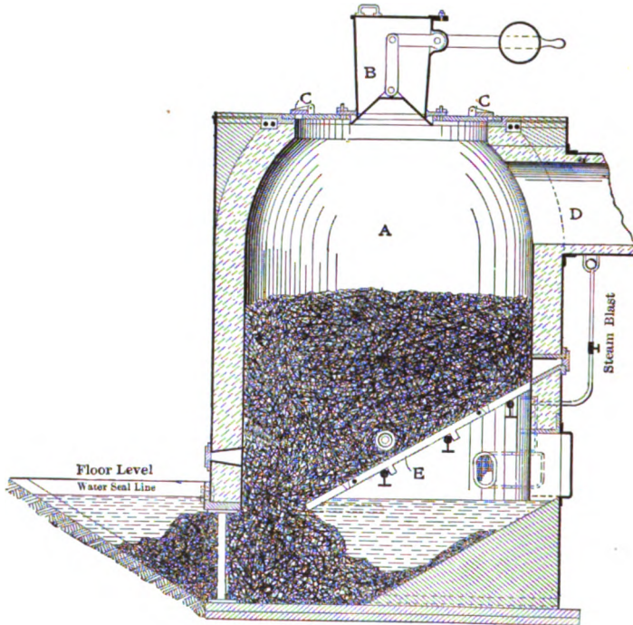
FIG. 30. — SMYTHE GAS-PRODUCER.
