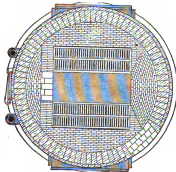
FIG. 24. — AMERICAN FURNACE AND MACHINE CO.'S PRODUCER.
