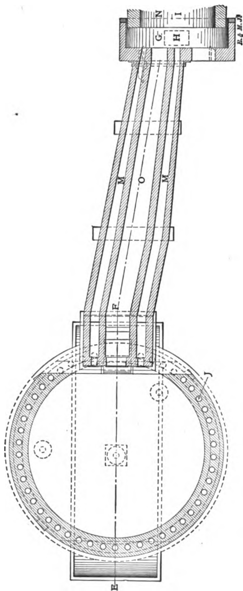
FIG. 94. — SWINDELL GAS-PRODUCER CONNECTED TO CEMENT KILN. (Sections A, B, C, D of Fig. 93.)
