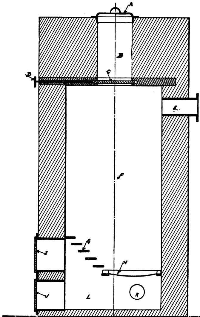
FIG. 17. — WEDDING PRODUCER.
