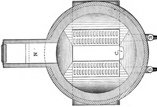
FIG. 28. — SWINDELL GAS-PRODUCER.
