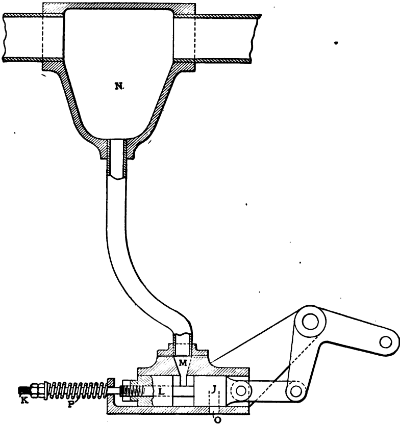
FIG. 71. — WYER WATER REGULATOR.
