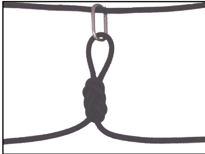
Figure 7-18. Hauling line.
