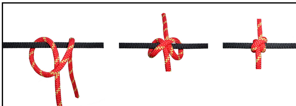
Figure 4-14. Clove hitch.
