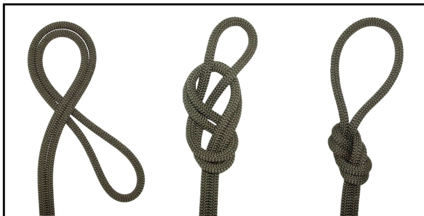
Figure 4-19. Figure-eight loop.
