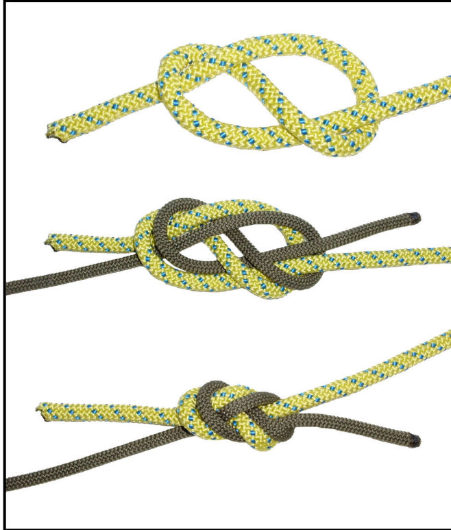
Figure 4-9. Figure-eight bend.
