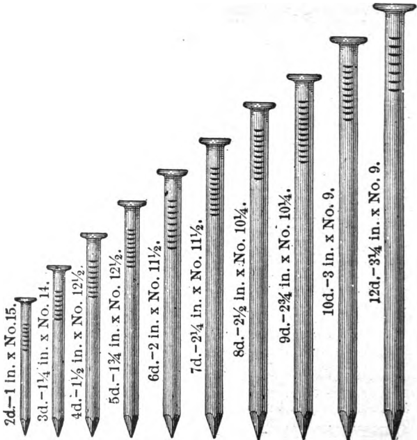
FIG. 235.—Wire nails.
