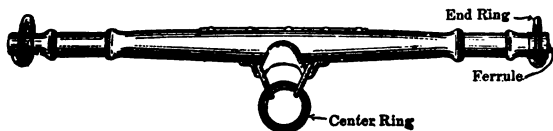
FIG. 150.—Neck yoke
