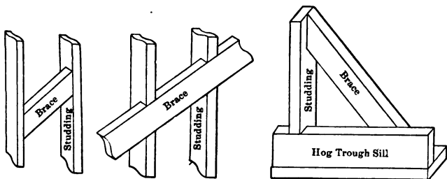
FIG. 78.—Studding braces.
