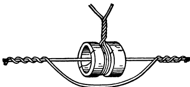
FIG. 39.—Swinging insulator.
