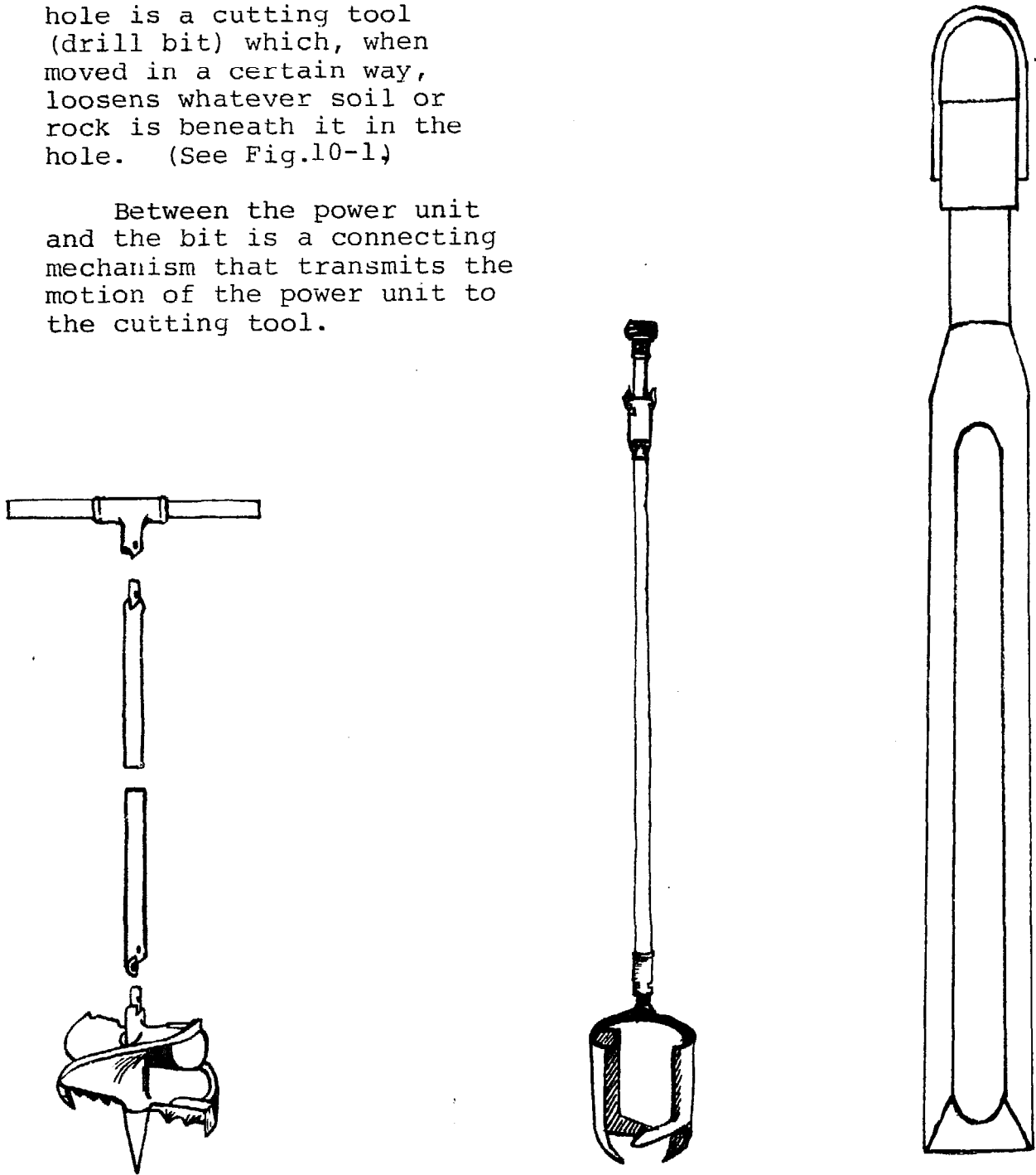
FIG. 10-1. DRILL BITS
