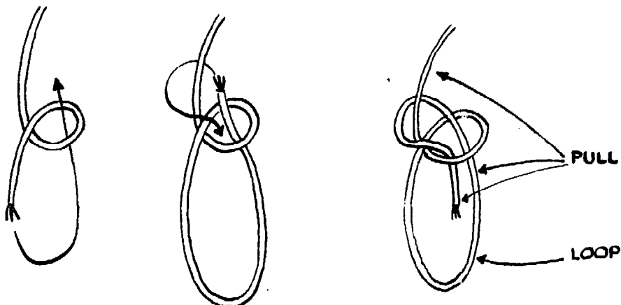
FIG.5-9. BOWLINE
