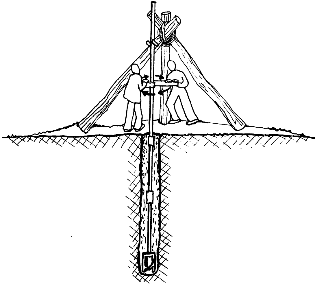
FIG. 11-3. HAND AUGERING
