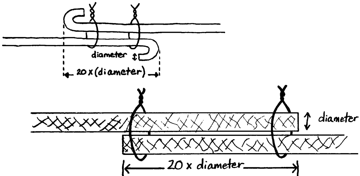
FIG. IV-4. REROD OVERLAP
