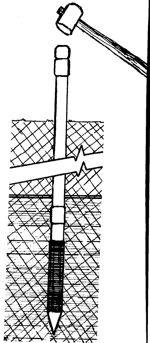
FIG. 11-7. DRIVEN WELL
