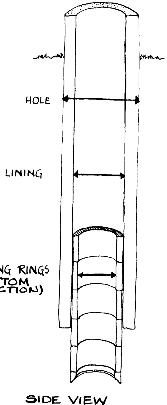
FIG. 3-4. THREE DIFFERENT WELL DIAMETERS USED DURING CONSTRUCTION.
