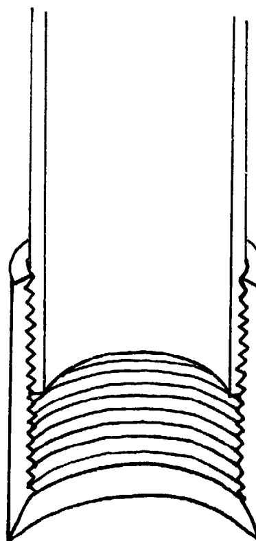
FIG. 13-2. SHARPENED COUPLING
