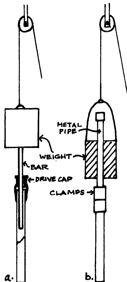
FIG. 14-8. HEAVY DRIVING WEIGHTS
