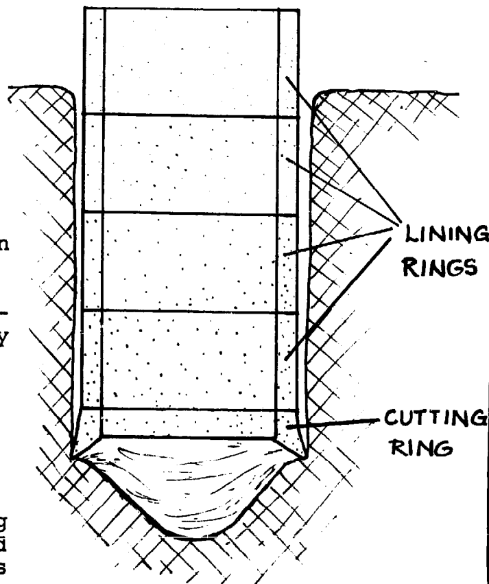
FIG. 7-1. SINK LINING
