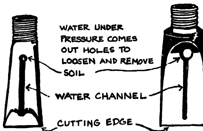
FIG. 14-12. JETTING BITS
